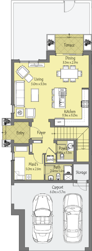
GROUND LEVEL
